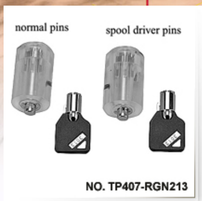
item no. TP407-RGN213 description. Visible Tubular Cylinder Set material.
