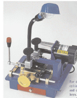
No. 707W Dimensions: (W)33x(D)31x(H)26cm N. W.: 16kg Motor: AC:110V or 220/240V 50Hz or 60Hz 60W
