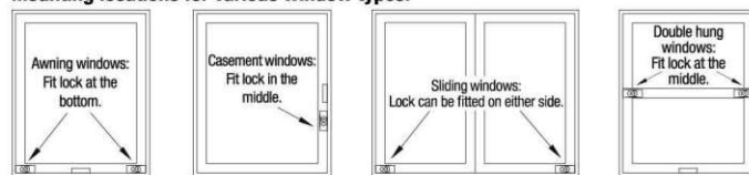
Mounting locations for various window types:
