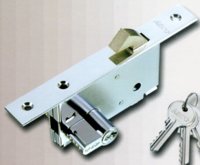
No. CH375/8 Mortise Lock Latch Type with flat type bolt with profile cylinder
