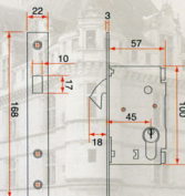
No. TN75-705 Mortise Lock with hook type bolt with profile cylinder
