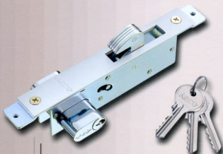
No. CH375/4 Mortise Lock with hook type bolt with light duty oval type cylinder
