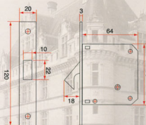
No. TN75/6 Mortise Lock with hook type bolt with cross keys
